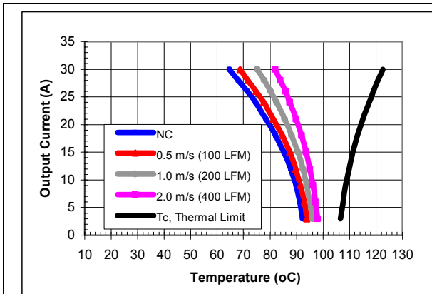
iQE24030A033V-000 maximum output current vs. ambient temperature at nominal input voltage for airflow rates natural convection (60lfm) to 400lfm with airflow from pin 3 to pin 1 (best orientation).
