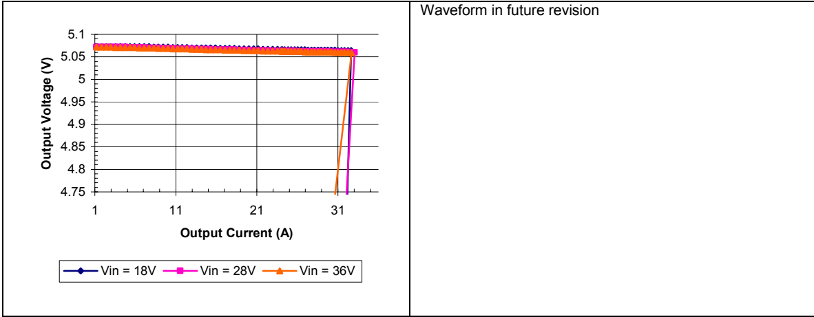
iQE24024A050V-000 Typical Output Current Limit Characteristics vs. Input Voltage at Ta=25 degrees.
