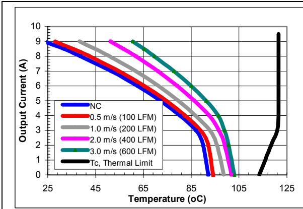
iQE24009A120V-000 maximum output current vs. ambient temperature at nominal input voltage for airflow rates natural convection (60lfm) to 600lfm with airflow from pin 3 to pin 1 (best orientation).
