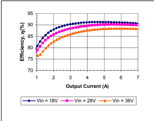
iQE24007A150V-000 Typical Efficiency vs. Input Voltage at Ta=25 degrees.
