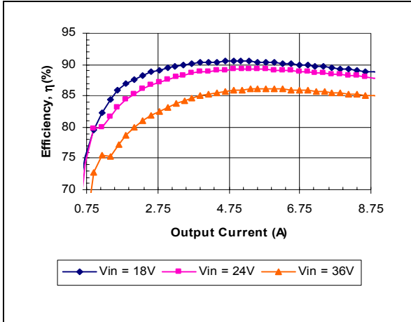
iQE24009A120V-000 Typical Efficiency vs. Input Voltage at Ta=25 degrees.
