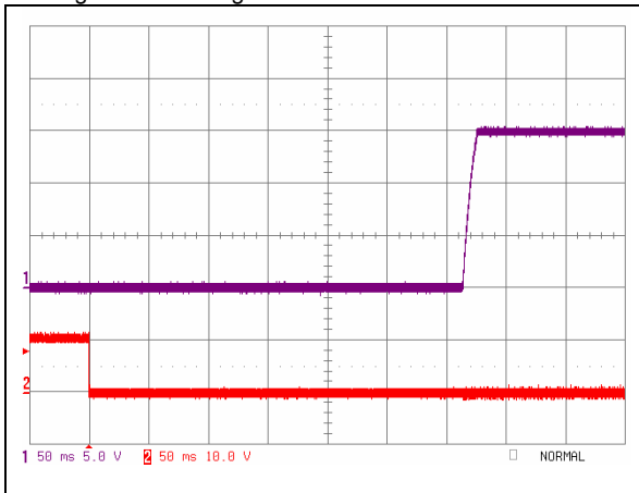
iQE24007A150V-001 Typical startup characteristic from on/off at full load. Lower trace - on/off signal, Upper trace – output voltage 5V/div. Time scale 50mS/div.
