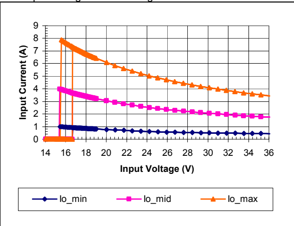
iQE24012A080V-000 Typical Input Current vs. Input Voltage Characteristics
