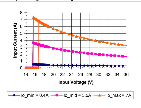
iQE24007A150V-000 Typical Input Current vs. Input Voltage Characteristics
