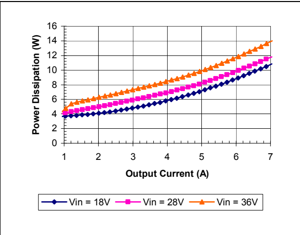
iQE24007A150V-000 Typical Power Dissipation vs. Input Voltage at Ta=25 degrees
