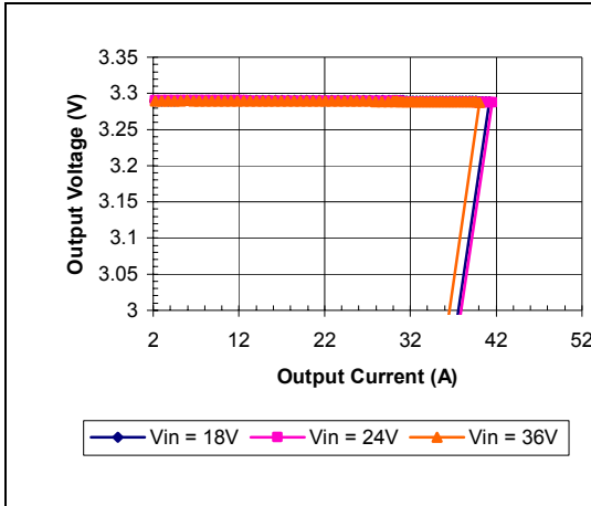
iQE24030A033V-000 Typical Output Current Limit Characteristics vs. Input Voltage at Ta=25 degrees.
