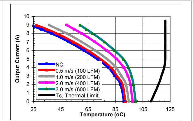
iQE24009A120V-000 maximum output current vs. ambient temperature at nominal input voltage for airflow rates natural convection (60lfm) to 600lfm with airflow from pin 1 to pin 3
