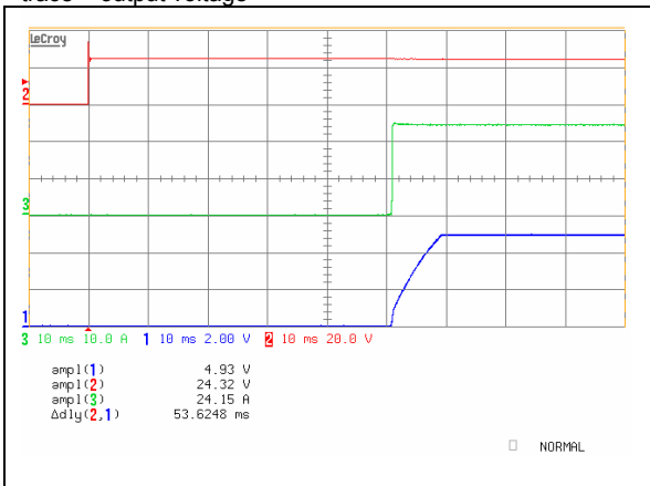
iQE24024A050V-000 Typical startup characteristic from input voltage application at full load. Upper trace - input voltage, lower trace – output voltage
