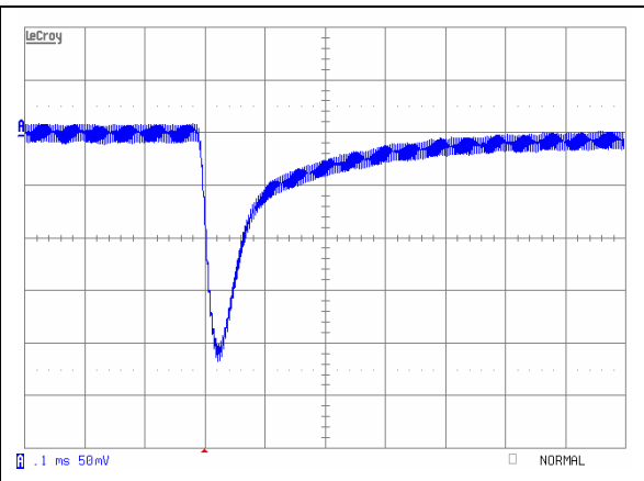
iQE24012A080V-000 Typical transient response. Output voltage response to load step from 50% to 75% of full load with output current slew rate of 0.1A/uS.
