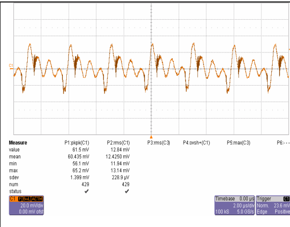
iQE24012A080V-000 Typical Output Ripple at nominal Input voltage and full load at Ta=25 degree, 20mV/div
