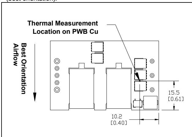
iQE24024A050V-000 thermal measurement location – top view
