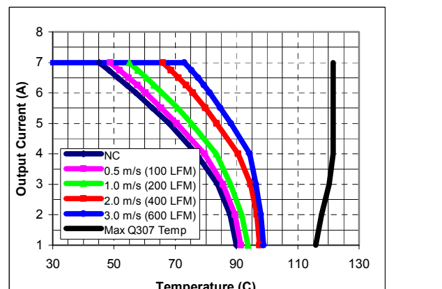
iQE24007A150V-000 maximum output current vs. ambient temperature at nominal input voltage for airflow rates natural convection (60lfm) to 600lfm with airflow from pin 1 to pin 3
