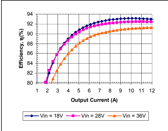
iQE24012A080V-000 Typical Efficiency vs. Input Voltage at Ta=25 degrees.
