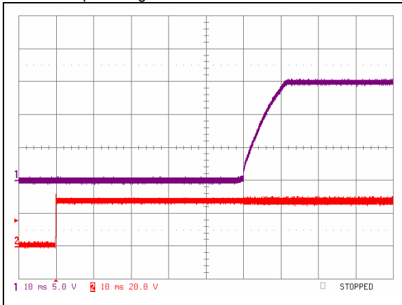
iQE24007A150V-000 Typical startup from input voltage application at full load. Lower trace - input voltage, Upper trace – output voltage. Time scale 10ms/div.
