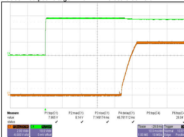
iQE24012A080V-000 Typical startup from input voltage application at full load. Upper trace - input voltage, lower trace – output voltage. Time scale 10ms/div
