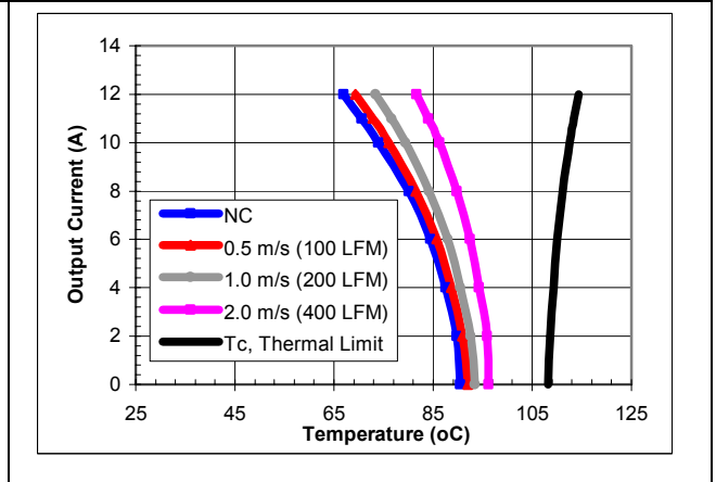
iQE24012A080V-000 maximum output current vs. ambient temperature at nominal input voltage for airflow rates natural convection (60lfm) to 400lfm with airflow from pin 1 to pin 3
