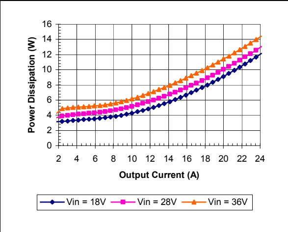
iQE24024A050V-000 Typical Power Dissipation vs. Input Voltage at Ta=25 degrees
