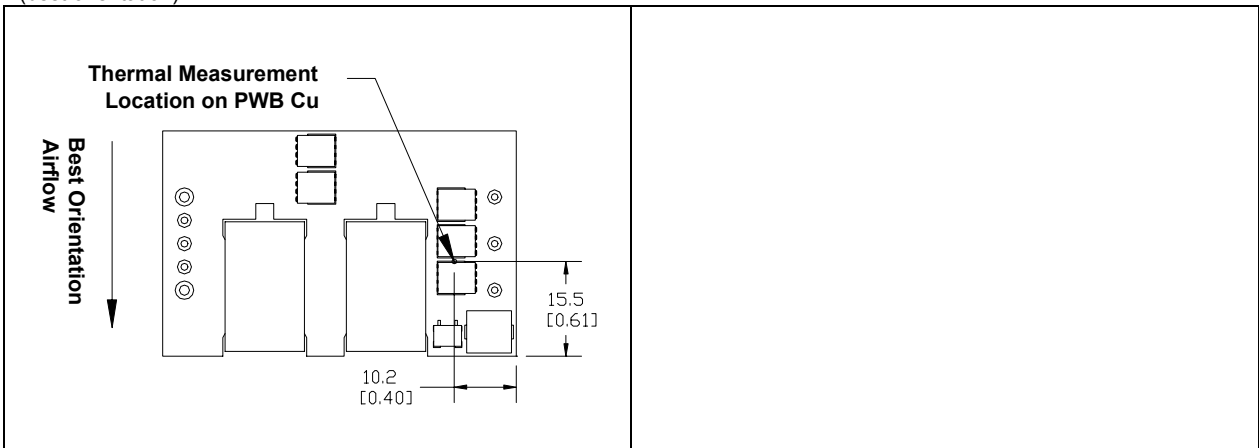
iQE24012A080V-000 thermal measurement location – top view
