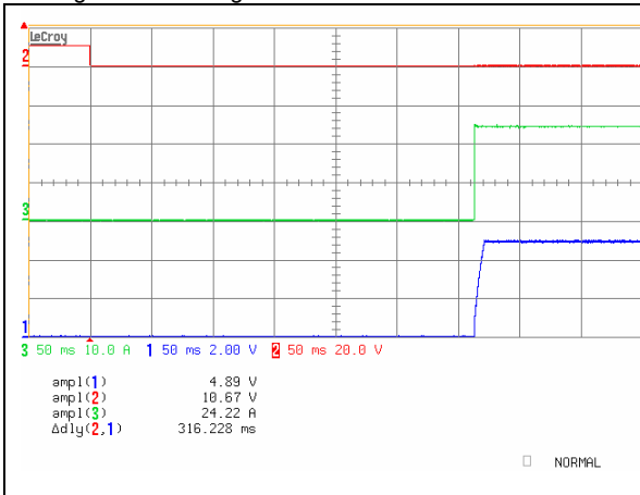
iQE24024A050V-001 Typical startup characteristic from on/off at full load. Upper trace - on/off signal, lower trace – output voltage
