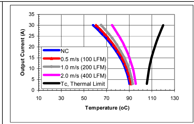
iQE24030A033V-000 maximum output current vs. ambient temperature at nominal input voltage for airflow rates natural convection (60lfm) to 400lfm with airflow from pin 1 to pin 3
