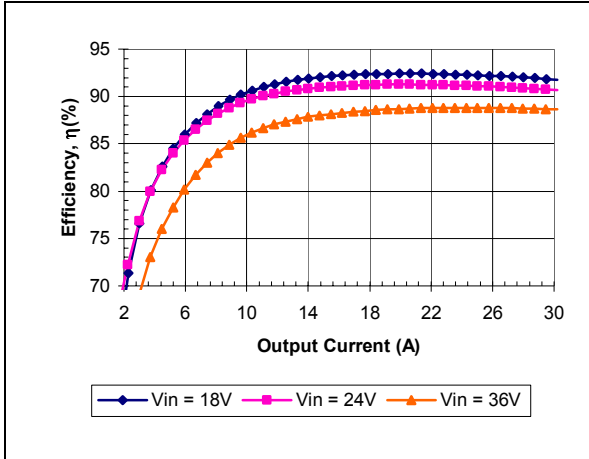
iQE24030A033V-000 Typical Efficiency vs. Input Voltage at Ta=25 degrees.
