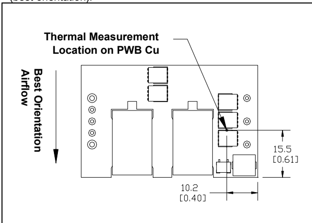
iQE24007A150V-000 thermal measurement location – top view
