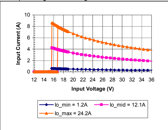
iQE24024A050V-000 Typical Input Current vs. Input Voltage Characteristics
