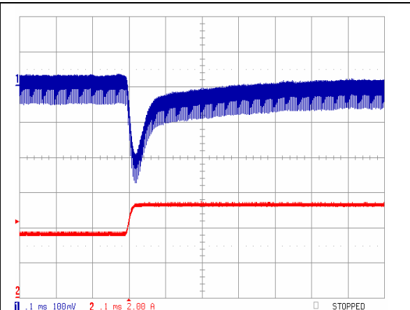
iQE24007A150V-000 Typical output voltage response to load step from 50% to 75% of full load with output current slew rate of 0.1A/uS. 100mV, 100uS per div.
