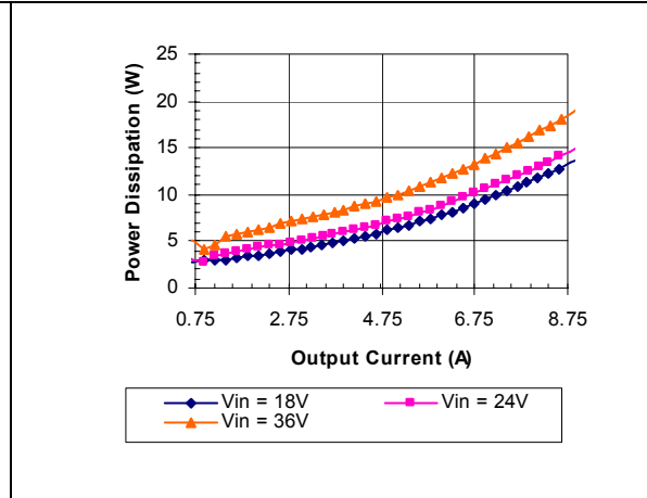
iQE24009A120V-000 Typical Power Dissipation vs. Input Voltage at Ta=25 degrees
