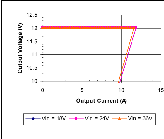
iQE24009A120V-000 Typical Output Current Limit Characteristics vs. Input Voltage at Ta=25 degrees.
