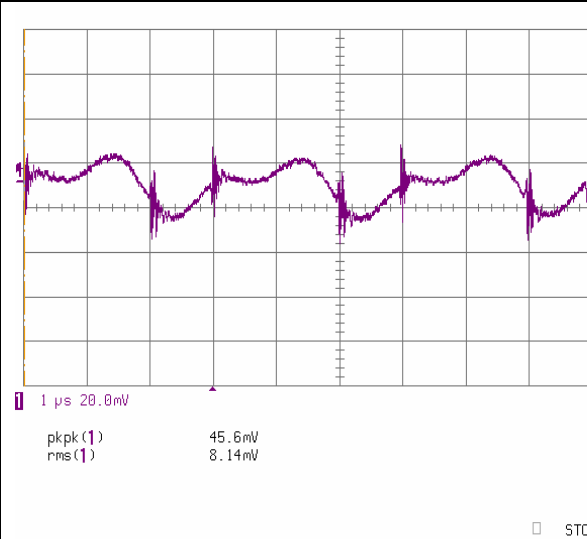
iQE24007A150V-000 Typical Output Ripple at nominal Input voltage and full load at Ta=25 degree
