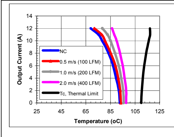
iQE24012A080V-000 maximum output current vs. ambient temperature at nominal input voltage for airflow rates natural convection (60lfm) to 400lfm with airflow from pin 3 to pin 1 (best orientation).
