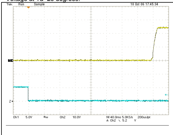
iQE24009A120V-001 Typical startup characteristic from on/off at full load. Lower trace - on/off signal, Upper trace – output voltage 5V/div. Time scale 40mS/div.
