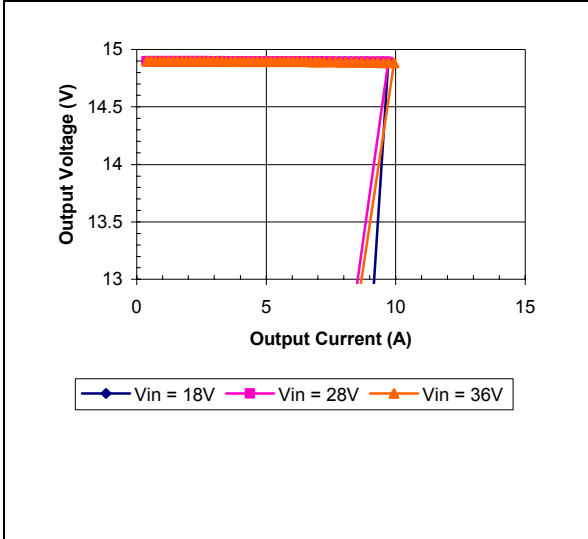
iQE24007A150V-000 Typical Output Current Limit Characteristics vs. Input Voltage at Ta=25 degrees.
