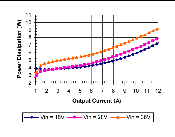
iQE24012A080V-000 Typical Power Dissipation vs. Input Voltage at Ta=25 degrees
