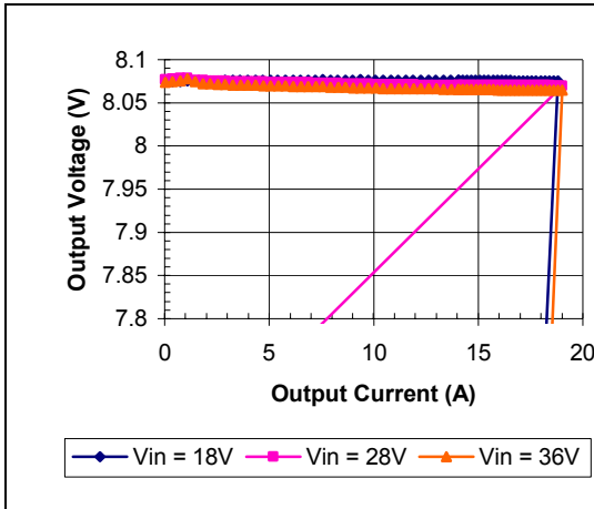
iQE24012A080V-000 Typical Output Current Limit Characteristics vs. Input Voltage at Ta=25 degrees.
