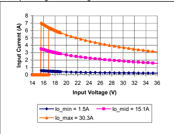
iQE24030A033V-000 Typical Input Current vs. Input Voltage Characteristics
