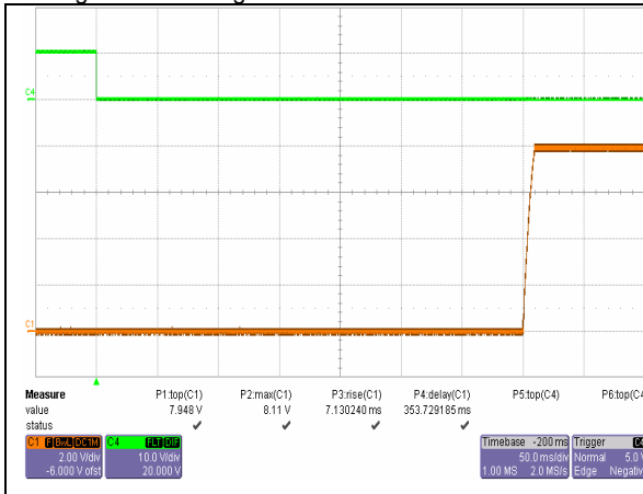
iQE24012A080V-001 Typical startup characteristic from on/off at full load. Upper trace - on/off signal, lower trace – output voltage 2V/div. Time scale 50ms/div.
