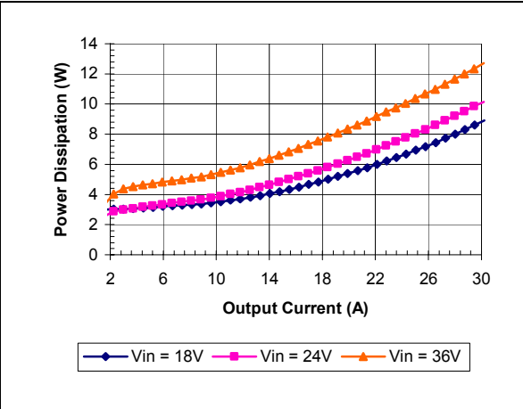
iQE24030A033V-000 Typical Power Dissipation vs. Input Voltage at Ta=25 degrees
