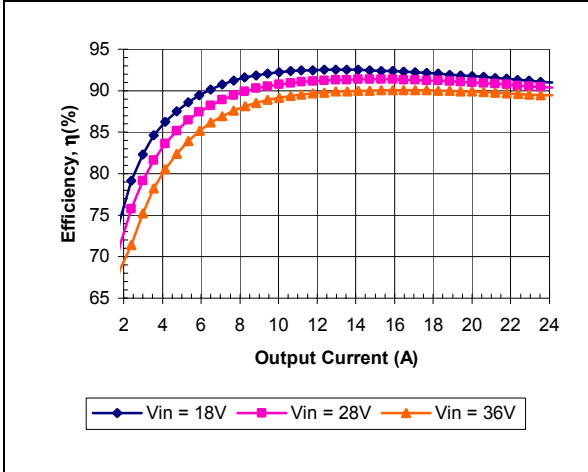
iQE24024A050V-000 Typical Efficiency vs. Input Voltage at Ta=25 degrees.
