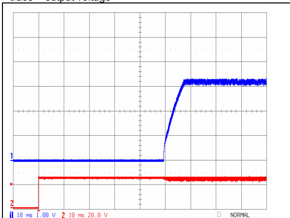
iQE24030A033V-000 Typical startup characteristic from input voltage application at full load. Upper trace - output voltage, lower trace – input voltage
