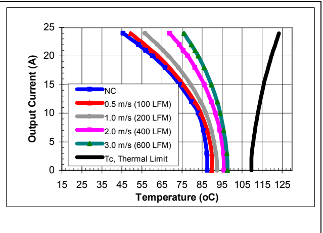
iQE24024A050V-000 maximum output current vs. ambient temperature at nominal input voltage for airflow rates natural convection (60lfm) to 600lfm with airflow from pin 1 to pin 3
