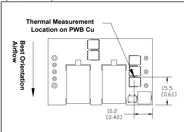
iQE24009A120V-000 thermal measurement location – top view
