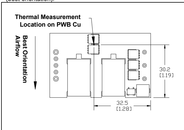
iQE24030A033V-000 thermal measurement location – top view
