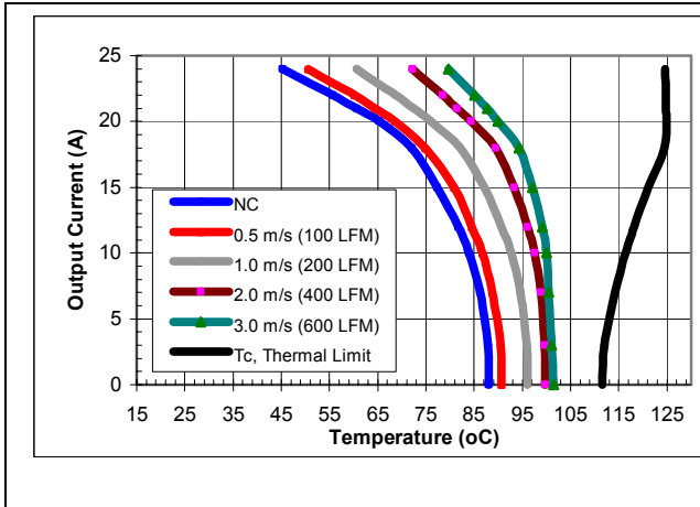
iQE24024A050V-000 maximum output current vs. ambient temperature at nominal input voltage for airflow rates natural convection (60lfm) to 600lfm with airflow from pin 3 to pin 1 (best orientation).
