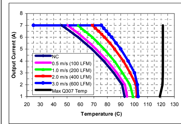
iQE24007A150V-000 maximum output current vs. ambient temperature at nominal input voltage for airflow rates natural convection (60lfm) to 600lfm with airflow from pin 3 to pin 1 (best orientation).
