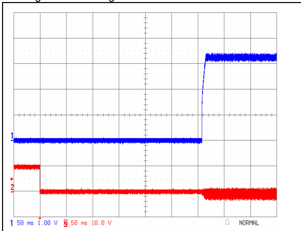
iQE24030A033V-001 Typical startup characteristic from on/off at full load. Lower trace - on/off signal, upper trace – output voltage
