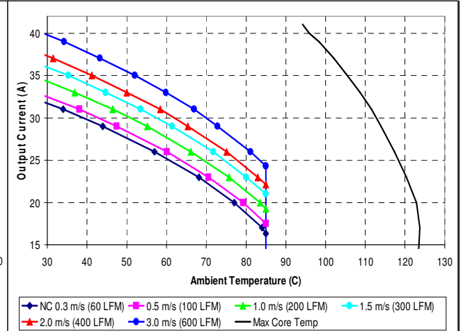
Maximum output current vs. ambient temperature at nominal input voltage with no base plate for airflow rates natural convection (0.3m/s) to 3.0m/s with airflow from pin 1 to pin 3.
