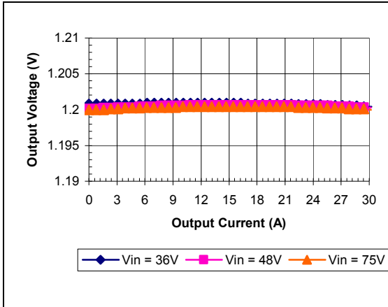
iSA48030A012V-000 Typical Output Voltage vs. Load Current at T_a = 25 degrees
