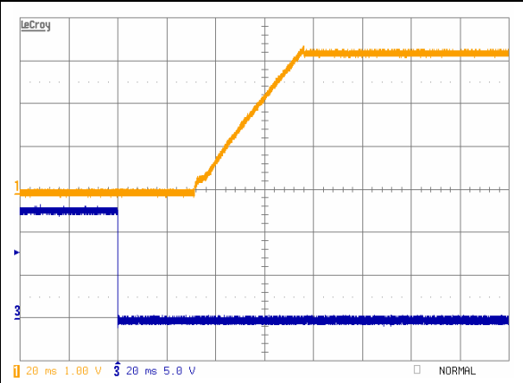
iSA48025A033V-001 Typical startup characteristic from on/off at full load. Ch3 - on/off signal 5V/div, Ch 1 – output voltage 1V/div; 20mS/div.
