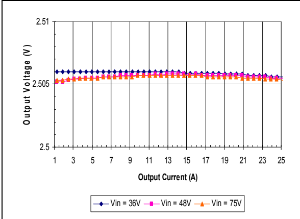
iSA48025A025V-000 Typical Output Voltage vs. Load Current at Ta = 25 degrees
