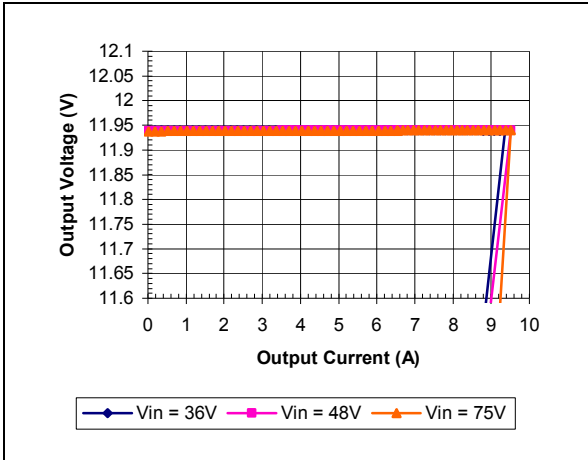
iSA48007A120V-000 Typical Output Current Limit Characteristics vs. Input Voltage at T_a=25 degrees.
