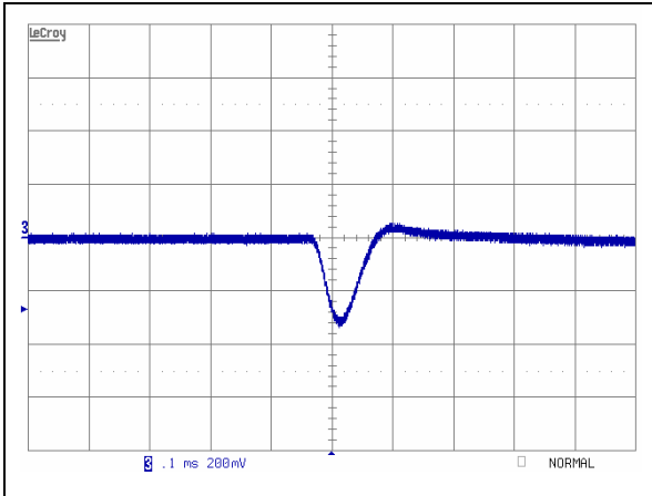
iSA48015A050V-000 Typical Output voltage response to load step from 50% to 75% of full load with output current slew rate of 0.1A/uS, 200mV/div and 0.1mS/div.
