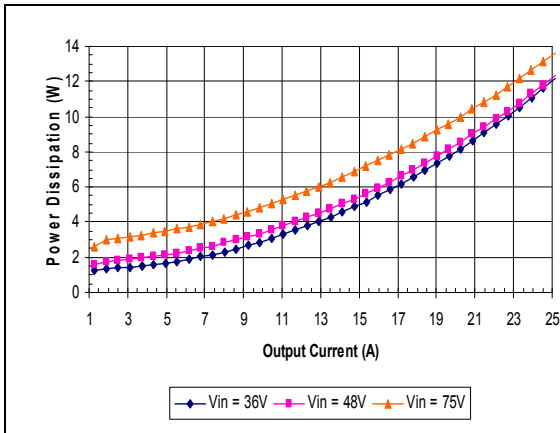
iSA48025A025V-000 Typical Power Dissipation vs. Input Voltage at Ta=85 degrees
