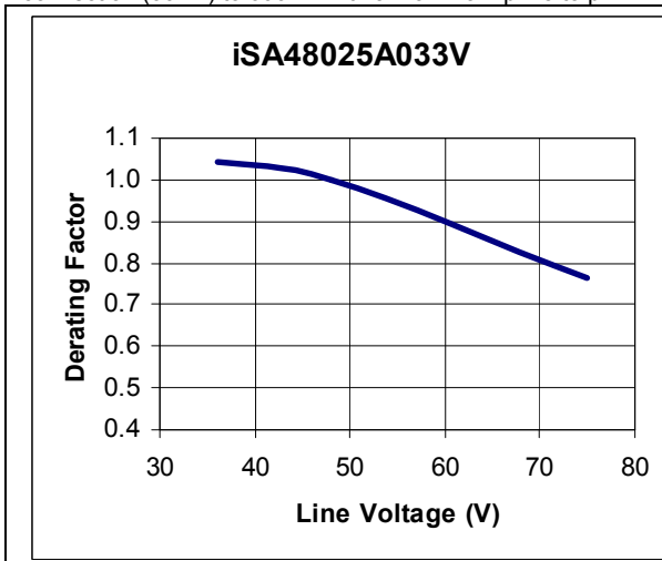
iSA48025A033V-000 typical temperature derating versus line voltage with 1m/s (200lfm) airflow
