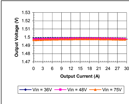
iSA48030A015V-000 Typical Output Voltage vs. Load Current at Ta = 25 degrees
