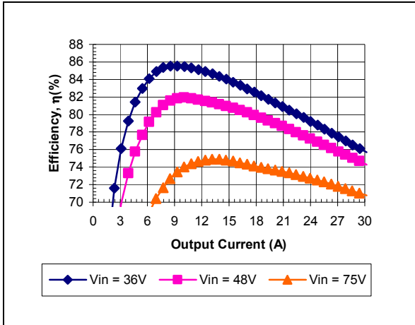
iSA48030A012V-000 Typical Efficiency vs. Input Voltage at Ta=25 degrees.
