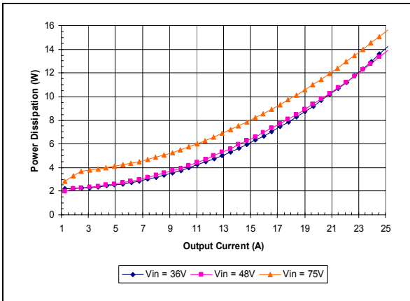
iSA48025A033V-000 Typical Power Dissipation vs. Input Voltage at Ta=85 degrees
