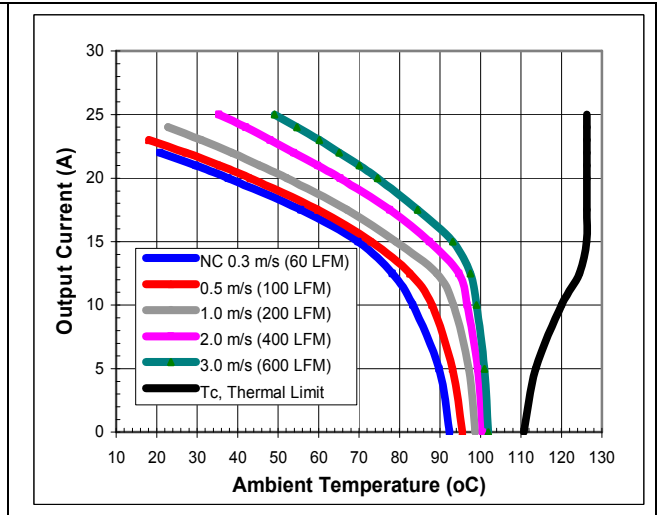
iSA48025A033V-000 maximum output current vs. ambient temperature at nominal input voltage for airflow rates natural convection (60lfm) to 600lfm with airflow from pin 1 to pin 3.
