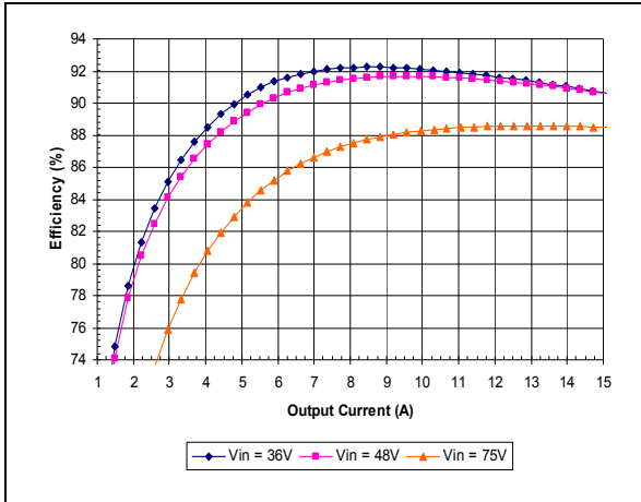
iSA48015A050V-000 Typical Efficiency vs. Input Voltage at Ta=25 degrees.
