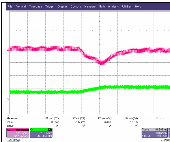
iSA48030A015V-000 Typical output voltage response to load step from 50% to 75% of full load with output current slew rate of 0.1A/uS.
