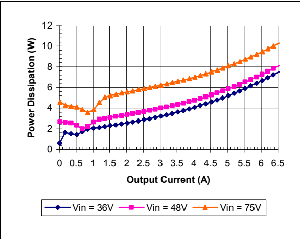
iSA48007A120V-000 Typical Power Dissipation vs. Input Voltage at Ta=25 degrees
