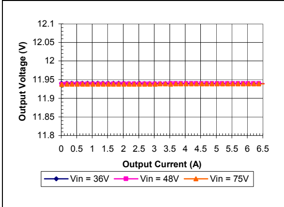
iSA48007A120V-000 Typical Output Voltage vs. Load Current at Ta = 25 degrees
