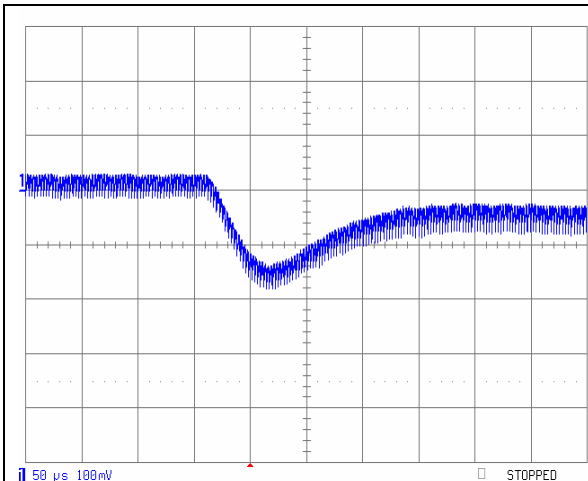
iSA48025A033V-000 Typical output voltage response to load step from 50% to 75% of full load with output current slew rate of 0.1A/uS, 100mV/div and 50uS/div.
