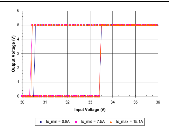
iSA48015A050V-000 Typical Output Voltage vs. Input Voltage Characteristics
