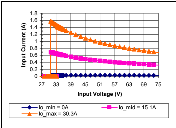
iSA48030A012V-000 Typical Input Current vs. Input Voltage Characteristics
