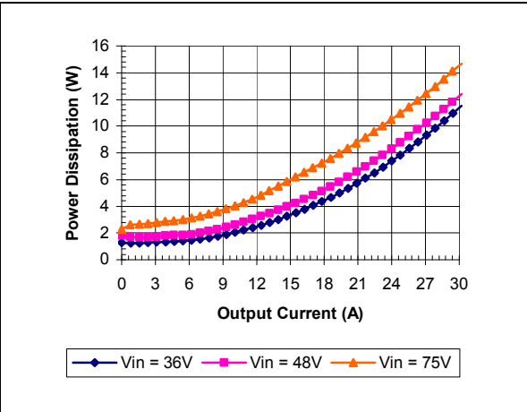
iSA48030A015V-000 Typical Power Dissipation vs. Input Voltage at Ta=25 degrees
