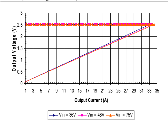
iSA48025A025V-000 Typical Output Current Limit Characteristics vs. Input Voltage at Ta=25 degrees.
