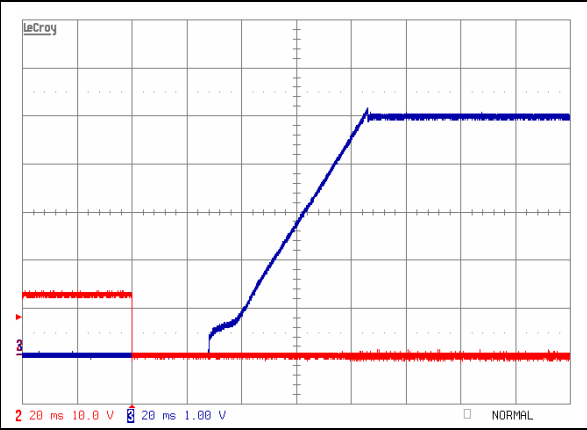
iSA48015A050V-001 Typical startup characteristic from on/off at full load. Ch2 - on/off signal 10V/div; Ch3 – output voltage 1V/div; 20mS/div time scale
