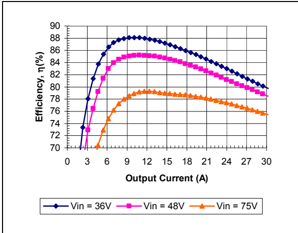
iSA48030A015V-000 Typical Efficiency vs. Input Voltage at Ta=25 degrees.
