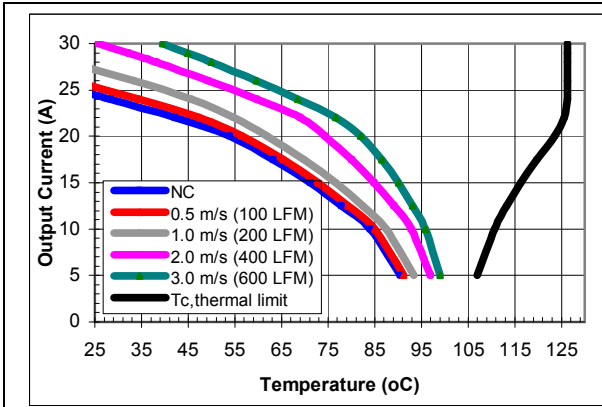
iSA48030A015V-000 maximum output current vs. ambient temperature at nominal input voltage for airflow rates natural convection (60lfm) to 600lfm with airflow from pin 3 to pin 1.
