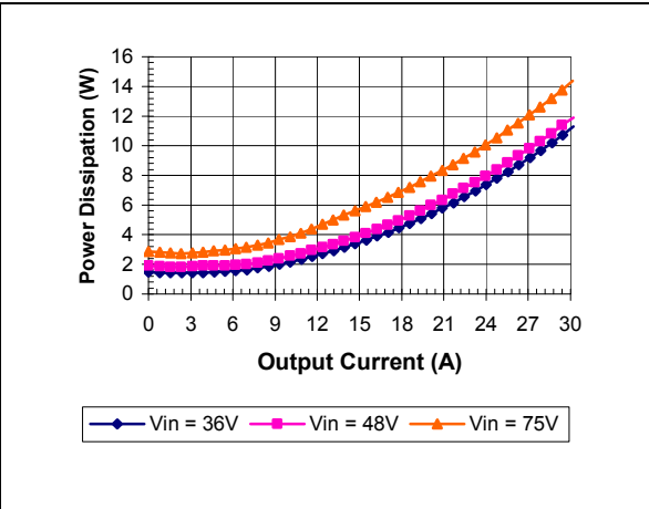
iSA48030A018V-000 Typical Power Dissipation vs. Input Voltage at Ta=25 degrees
