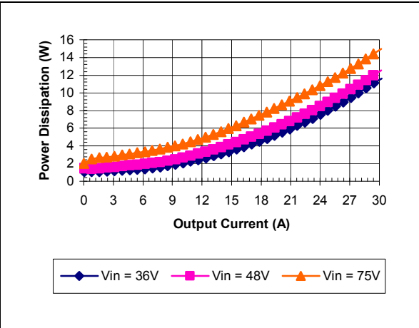
iSA48030A012V-000 Typical Power Dissipation vs. Input Voltage at Ta=25 degrees
