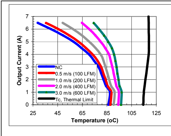
iSA48007A120V-000 maximum output current vs. ambient temperature at nominal input voltage for airflow rates natural convection (60lfm) to 600lfm with airflow from pin 3 to pin 1.
