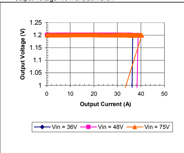
iSA48030A012V-000 Typical Output Current Limit Characteristics vs. Input Voltage at T_a=25 degrees.
