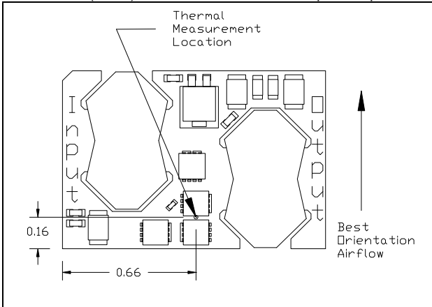
iSA48030A015V-000 thermal measurement location – top view
