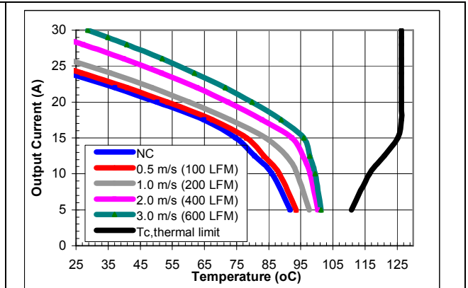
iSA48030A015V-000 maximum output current vs. ambient temperature at nominal input voltage for airflow rates natural convection (60lfm) to 600lfm with airflow from pin 1 to pin 3.
