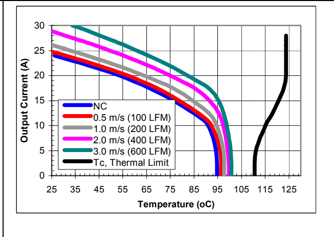
iSA48030A018V-000 maximum output current vs. ambient temperature at nominal input voltage for airflow rates natural convection (60lfm) to 600lfm with airflow from pin 1 to pin 3.
