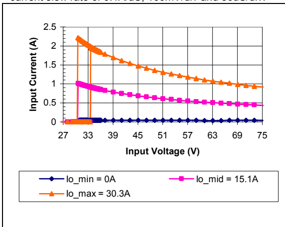
iSA48030A018V-000 Typical Input Current vs. Input Voltage Characteristics
