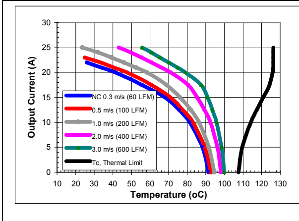
iSA48025A025V-000 maximum output current vs. ambient temperature at nominal input voltage for airflow rates natural convection (60lfm) to 600lfm with airflow from pin 3 to pin 1.
