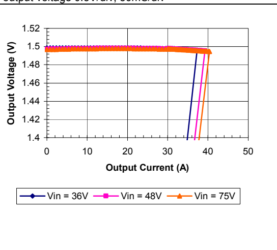
iSA48030A015V-000 Typical Output Current Limit Characteristics vs. Input Voltage at Ta=25 degrees.
