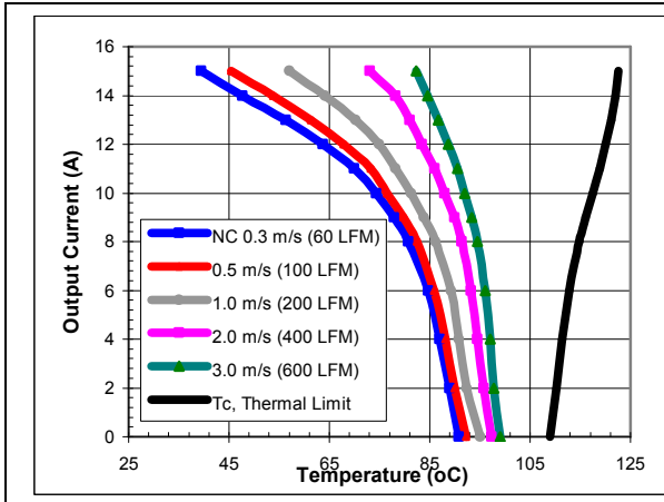
iSA48015A050V-000 maximum output current vs. ambient temperature at nominal input voltage for airflow rates natural convection (60lfm) to 600lfm with airflow from pin 3 to pin 1.
