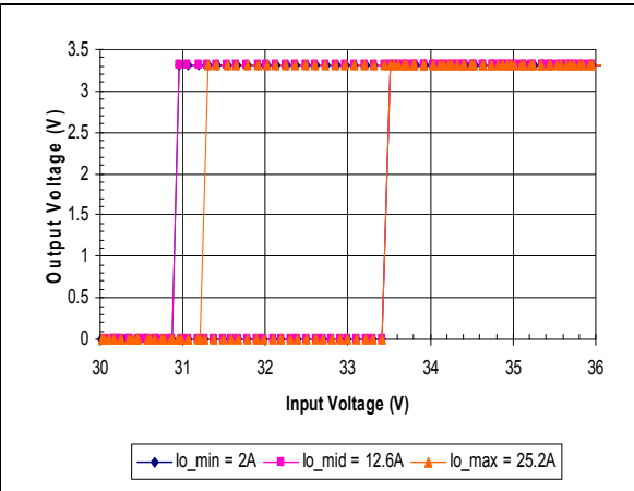
iSA48025A033V-000 Typical Output Voltage vs. Input Voltage Characteristics
