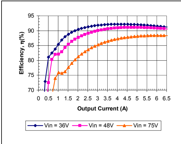
iSA48007A120V-000 Typical Efficiency vs. Input Voltage at Ta=25 degrees.
