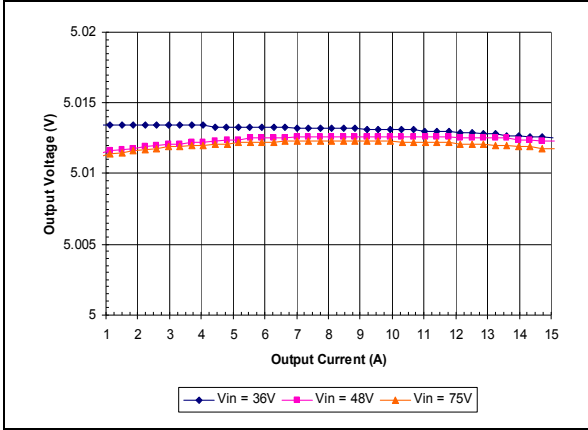
iSA48015A050V-000 Typical Output Voltage vs. Load Current at Ta = 25 degrees
