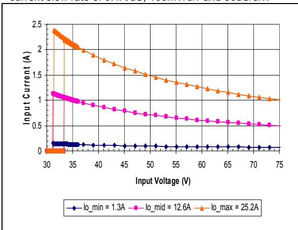
iSA48025A025V-000 Typical Input Current vs. Input Voltage Characteristics
