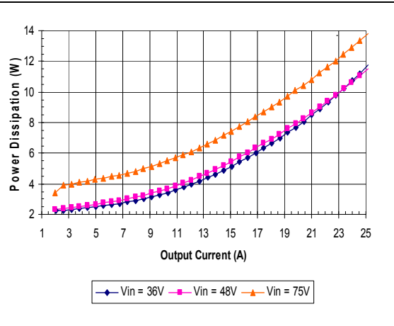
iSA48025A033V-000 Typical Power Dissipation vs. Input Voltage at Ta=25 degrees
