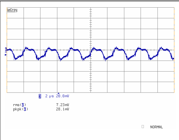
iSA48015A050V-000 Typical Output Ripple at nominal input voltage and full load at Ta=25 degrees; 20mV/div and 2uS/div.
