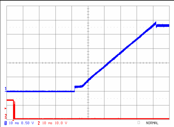
iSA48025A025V-001 Typical startup characteristic from on/off at full load. Ch2 - on/off signal 10V/div, Ch 1 – output voltage 0.5V/div; 10mS/div
