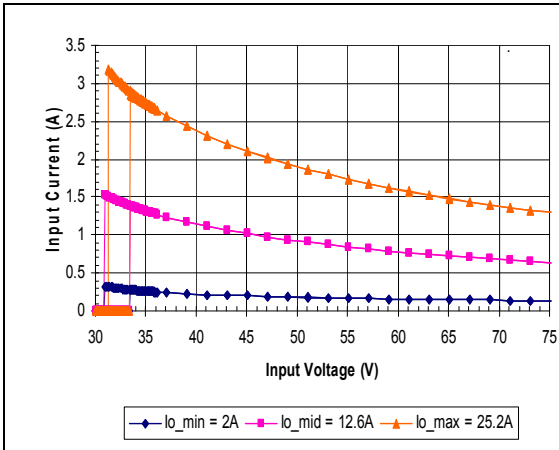
iSA48025A033V-000 Typical Input Current vs. Input Voltage Characteristics
