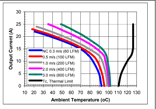
iSA48025A025V-000 maximum output current vs. ambient temperature at nominal input voltage for airflow rates natural convection (60lfm) to 600lfm with airflow from pin 1 to pin 3.
