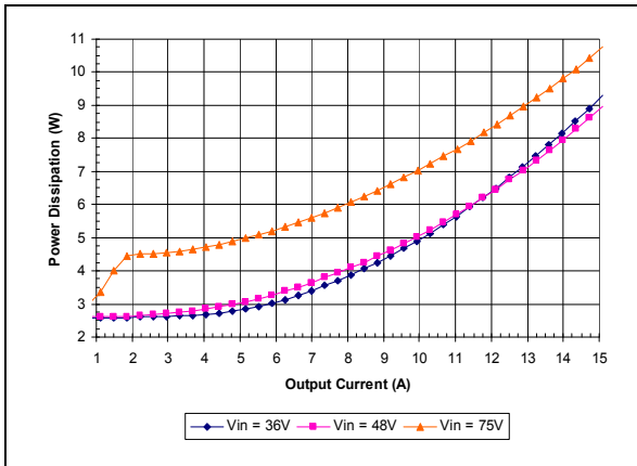
iSA48015A050V-000 Typical Power Dissipation vs. Input Voltage at Ta=85 degrees
