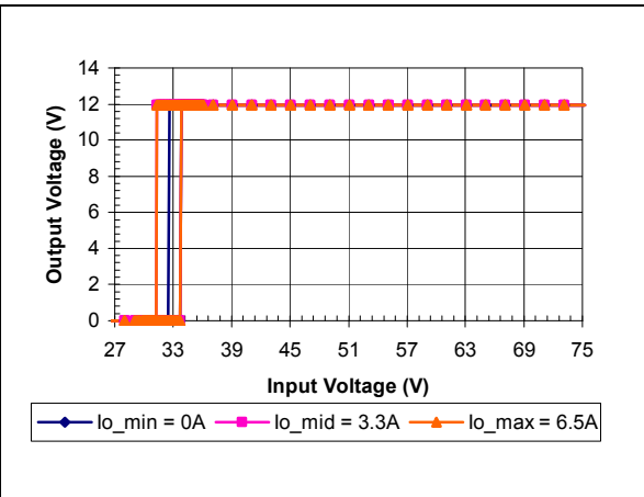
iSA48007A120V-000 Typical Output Voltage vs. Input Voltage Characteristics
