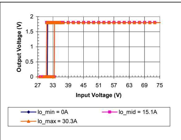
iSA48030A018V-000 Typical Output Voltage vs. Input Voltage Characteristics
