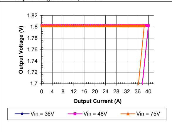
iSA48030A018V-000 Typical Output Current Limit Characteristics vs. Input Voltage at Ta=25 degrees.
