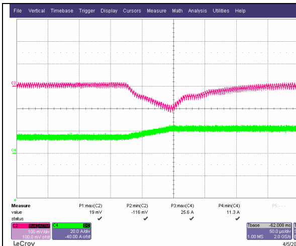
iSA48030A012V-000 Typical output voltage response to load step from 50% to 75% of full load with output current slew rate of 0.1A/uS.
