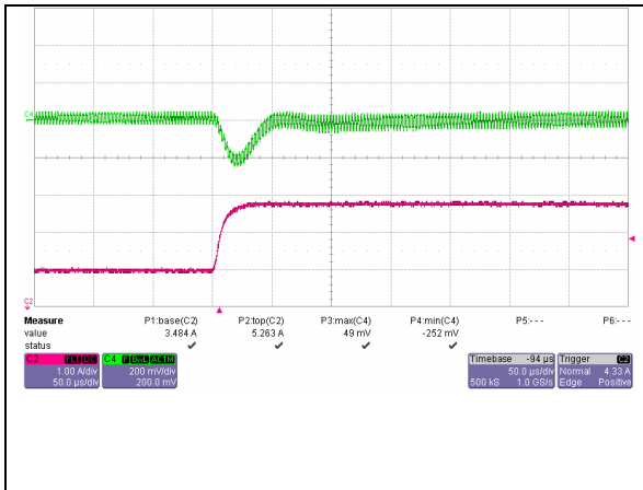
iSA48007A120V-000 Typical Output voltage response to load step from 50% to 75% of full load with output current slew rate of 0.1A/uS, 200mV/div and 50uS/div.
