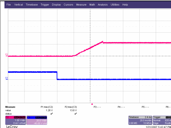
iSA48030A012V-001 Typical startup characteristic from on/off at full load. Ch3 - on/off signal 20V/div, Ch 2 – output voltage 1.0V/div; 20mS/div
