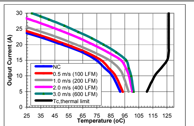
iSA48030A012V-000 maximum output current vs. ambient temperature at nominal input voltage for airflow rates natural convection (60lfm) to 600lfm with airflow from pin 1 to pin 3.
