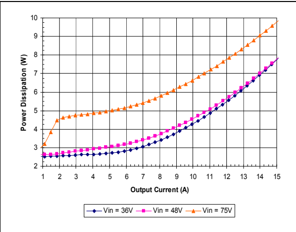
iSA48015A050V-000 Typical Power Dissipation vs. Input Voltage at Ta=25 degrees
