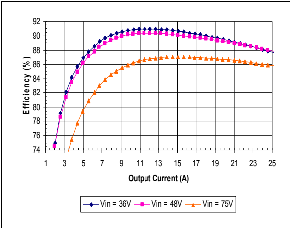
iSA48025A033V-000 Typical Efficiency vs. Input Voltage at Ta=25 degrees.
