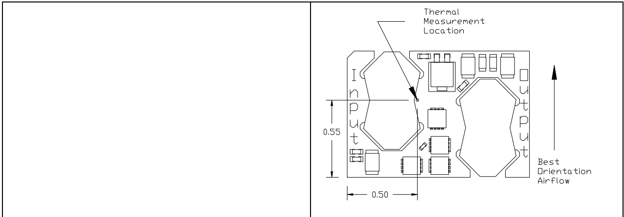
iSA48015A050V-000 thermal measurement location – top view
