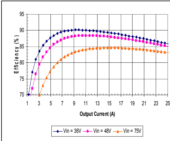
iSA48025A025V-000 Typical Efficiency vs. Input Voltage at Ta=25 degrees.
