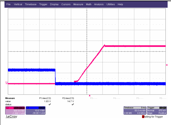
iSA48030A018V-001 Typical startup characteristic from on/off at full load. Ch3 - on/off signal 10V/div, Ch 2 – output voltage 0.5V/div; 50mS/div
