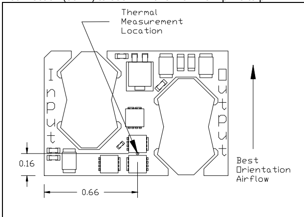
iSA48025A025V-000 thermal measurement location – top view
