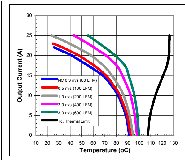
iSA48025A033V-000 maximum output current vs. ambient temperature at nominal input voltage for airflow rates natural convection (60lfm) to 600lfm with airflow from pin 3 to pin 1.
