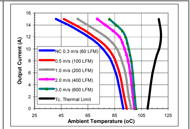
iSA48015A050V-000 maximum output current vs. ambient temperature at nominal input voltage for airflow rates natural convection (60lfm) to 600lfm with airflow from pin 1 to pin 3.
