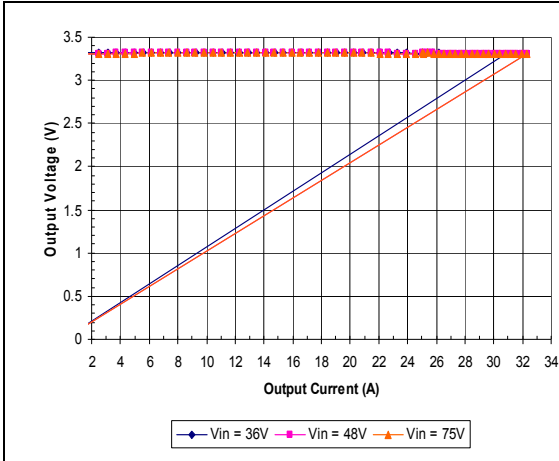
iSA48025A033V-000 Typical Output Current Limit Characteristics vs. Input Voltage at Ta=25 degrees.
