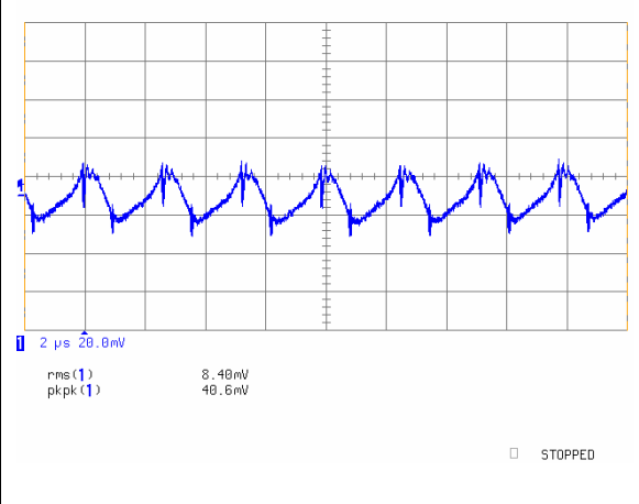
iSA48025A033V-000 Typical Output Ripple at nominal input voltage and full load at Ta=25 degrees; 20mV/div, 2µs/div.
