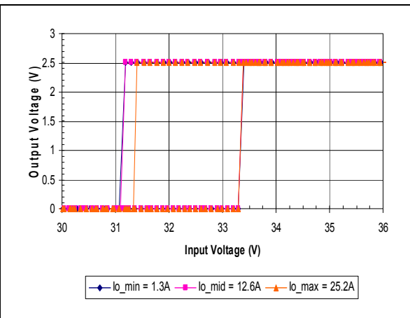
iSA48025A025V-000 Typical Output Voltage vs. Input Voltage Characteristics
