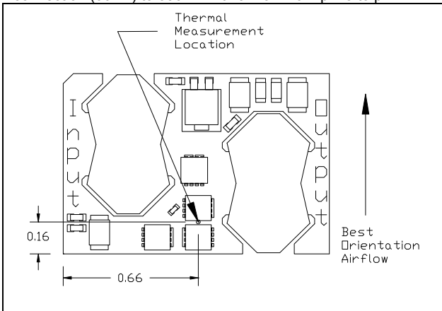
iSA48030A018V-000 thermal measurement location – top view
