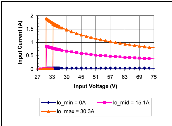
iSA48030A015V-000 Typical Input Current vs. Input Voltage Characteristics
