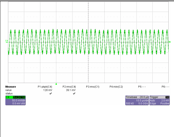
iSA48007A120V-000 Typical Output Ripple at nominal input voltage and full load at T_a=25 degrees; 50mV/div and 10uS/div.
