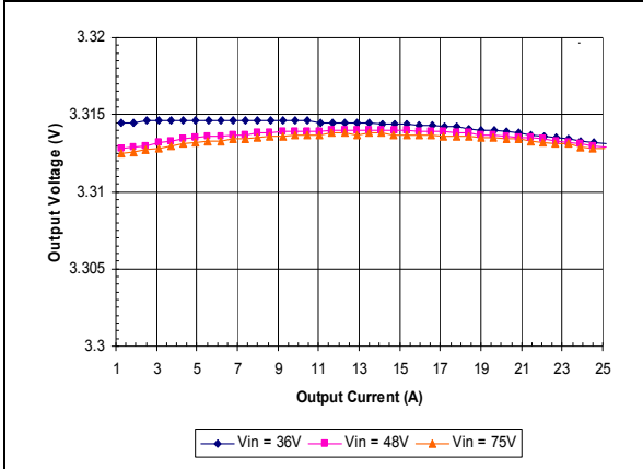
iSA48025A033V-000 Typical Output Voltage vs. Load Current at T_a = 25 degrees
