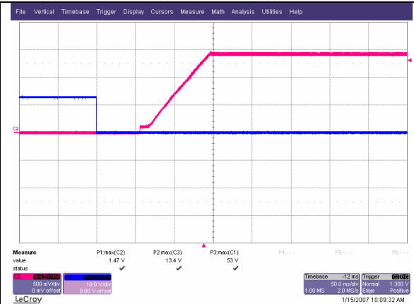
iSA48030A015V-001 Typical startup characteristic from on/off at full load. Ch3 - on/off signal 10V/div, Ch 2 – output voltage 0.5V/div; 50mS/div
