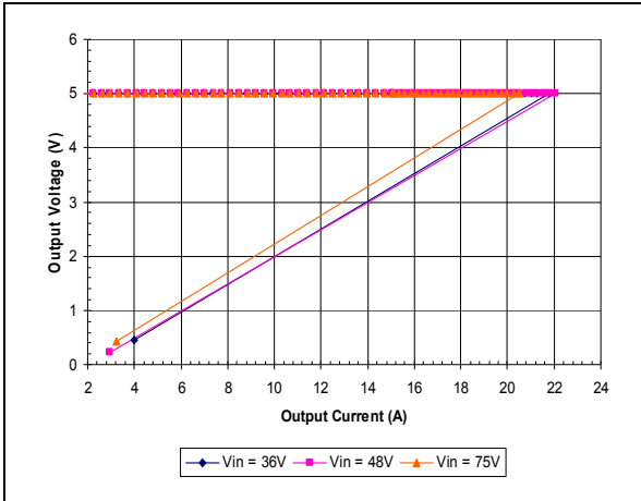
iSA48015A050V-000 Typical Output Current Limit Characteristics vs. Input Voltage at Ta=25 degrees.
