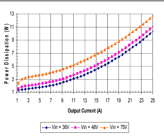
iSA48025A025V-000 Typical Power Dissipation vs. Input Voltage at Ta=25 degrees
