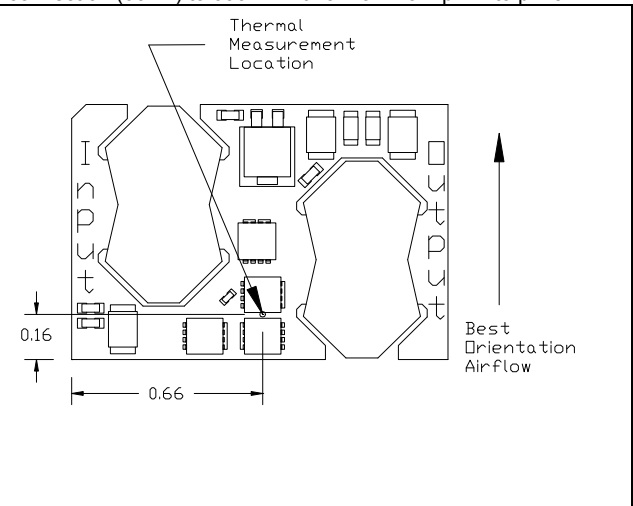
iSA48025A033V-000 thermal measurement location – top view
