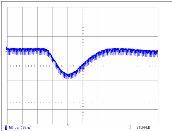
iSA48025A025V-000 Typical output voltage response to load step from 50% to 75% of full load with output current slew rate of 0.1A/uS, 100mV/div and 50uS/div.
