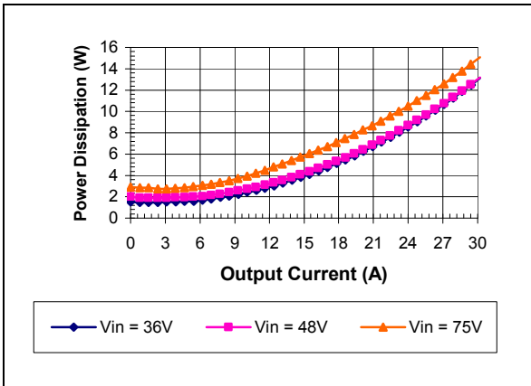
iSA48030A018V-000 Typical Power Dissipation vs. Input Voltage at Ta=85 degrees
