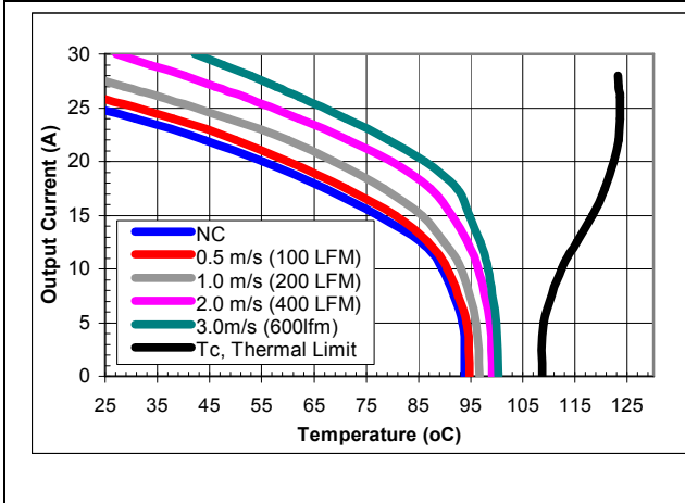
iSA48030A018V-000 maximum output current vs. ambient temperature at nominal input voltage for airflow rates natural convection (60lfm) to 600lfm with airflow from pin 3 to pin 1.
