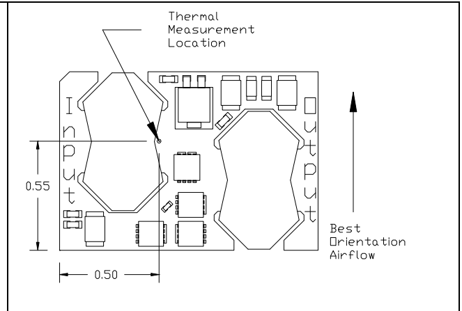
iSA48007A120V-000 thermal measurement location – top view
