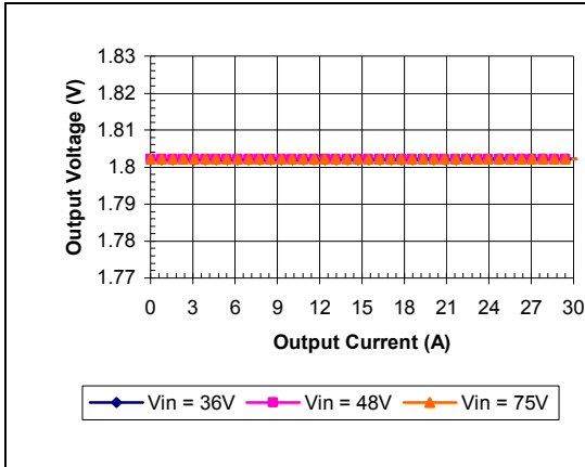
iSA48030A018V-000 Typical Output Voltage vs. Load Current at Ta = 25 degrees
