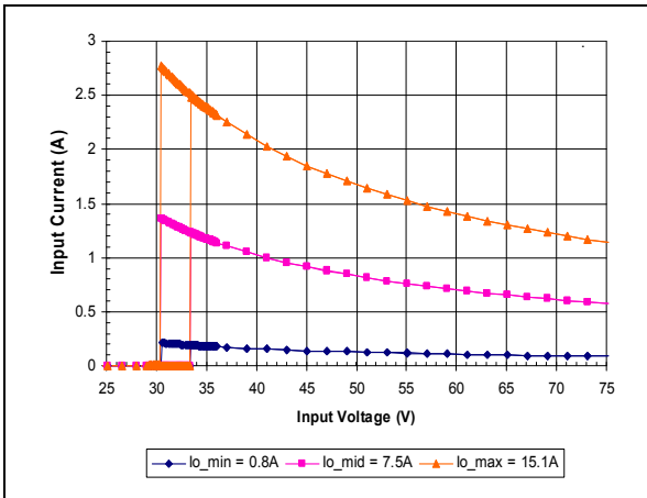
iSA48015A050V-000 Typical Input Current vs. Input Voltage Characteristics
