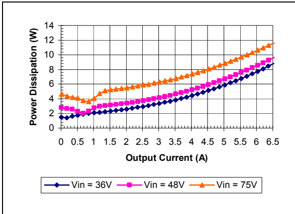
iSA48007A120V-000 Typical Power Dissipation vs. Input Voltage at Ta=85 degrees
