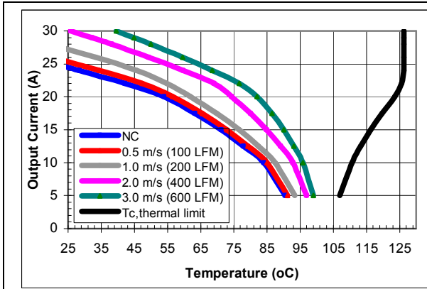
iSA48030A012V-000 maximum output current vs. ambient temperature at nominal input voltage for airflow rates natural convection (60lfm) to 600lfm with airflow from pin 3 to pin 1.
