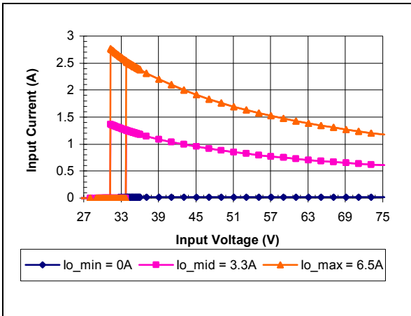
iSA48007A120V-000 Typical Input Current vs. Input Voltage Characteristics
