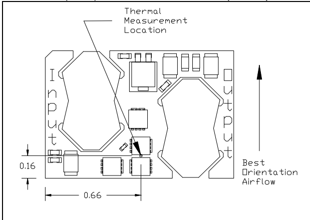
iSA48030A012V-000 thermal measurement location – top view
